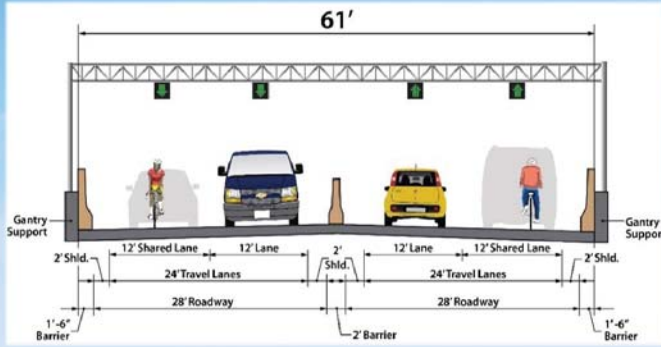
OPTION – LANE SHARING
