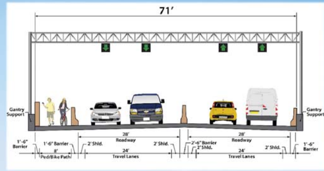
OPTION – SHARED USE PATH
