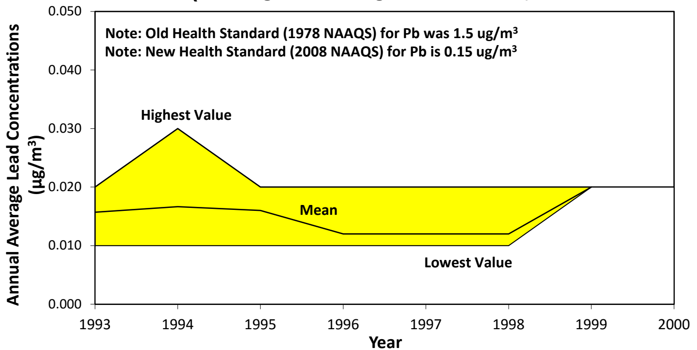
Figure 17: Annual Average Lead Concentrations (Washington, D.C. Region, 1993 - 2000)
