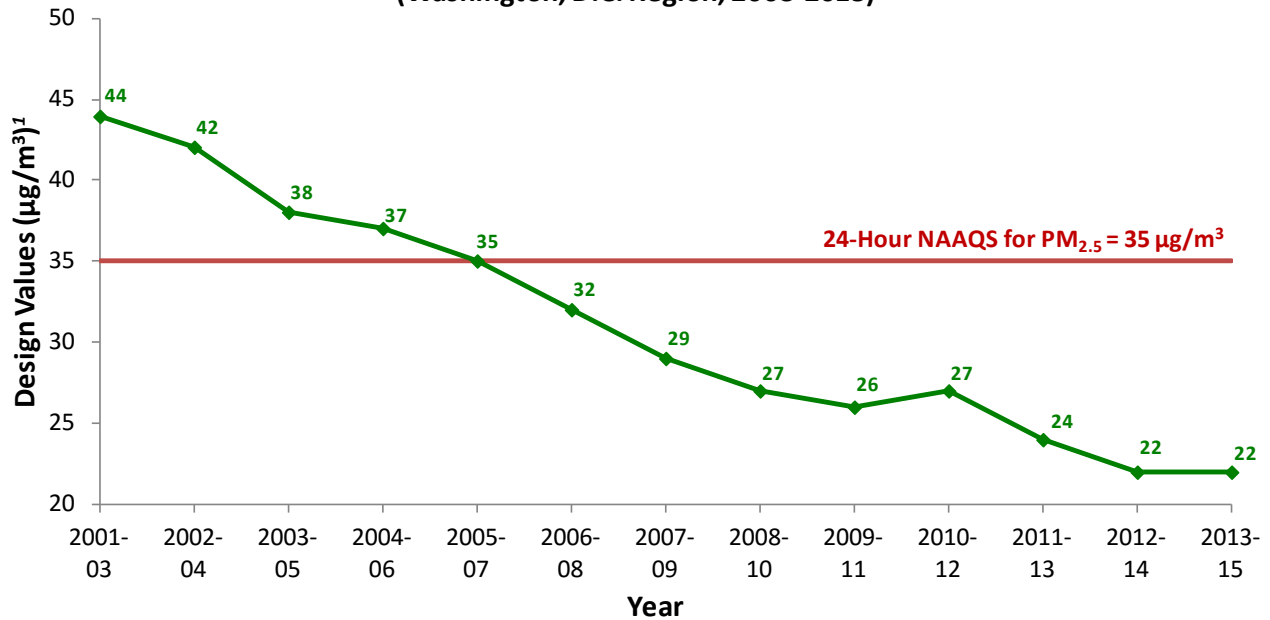
Figure 9: 24-Hour Design Values for PM 2.5 (Washington, D.C. Region, 2003-2015)
