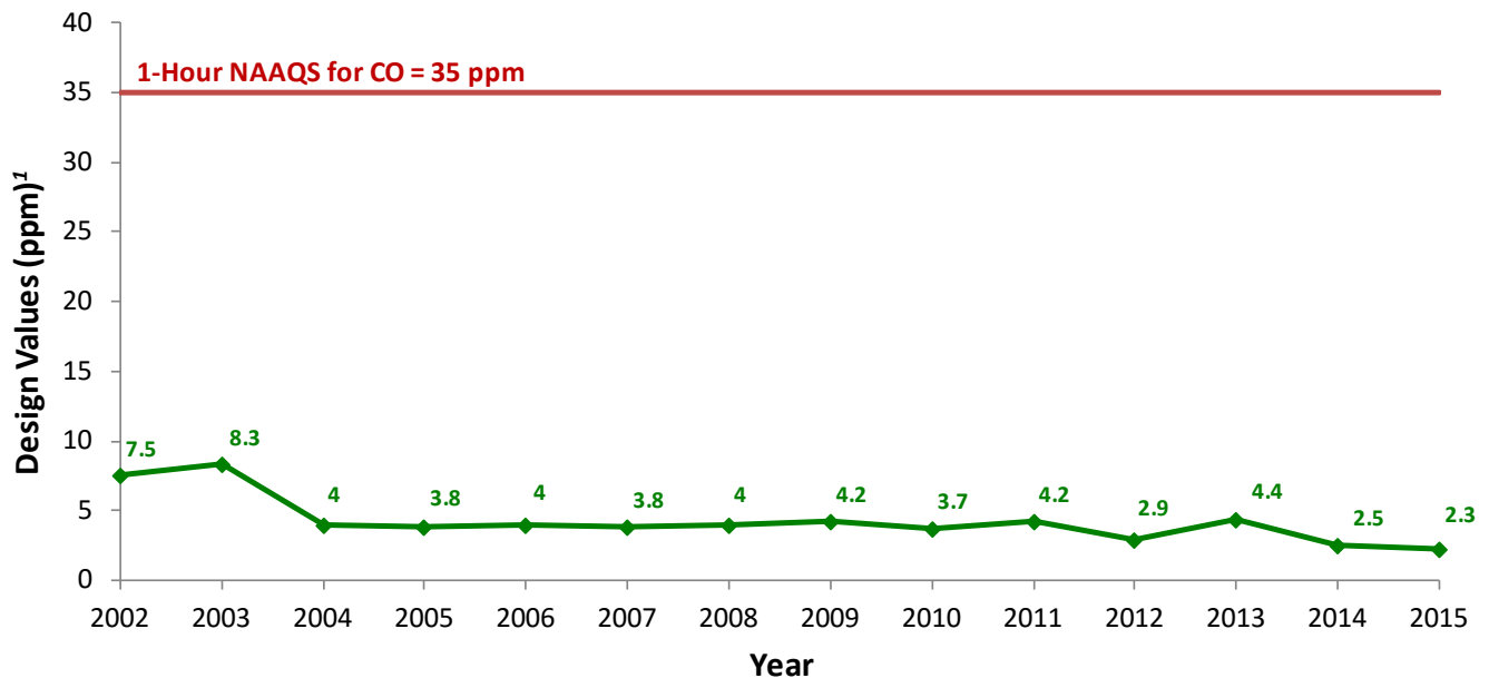
Figure 10: 1-Hour Design Values for Carbon Monoxide (Washington, D.C. Region, 2002-2015)
