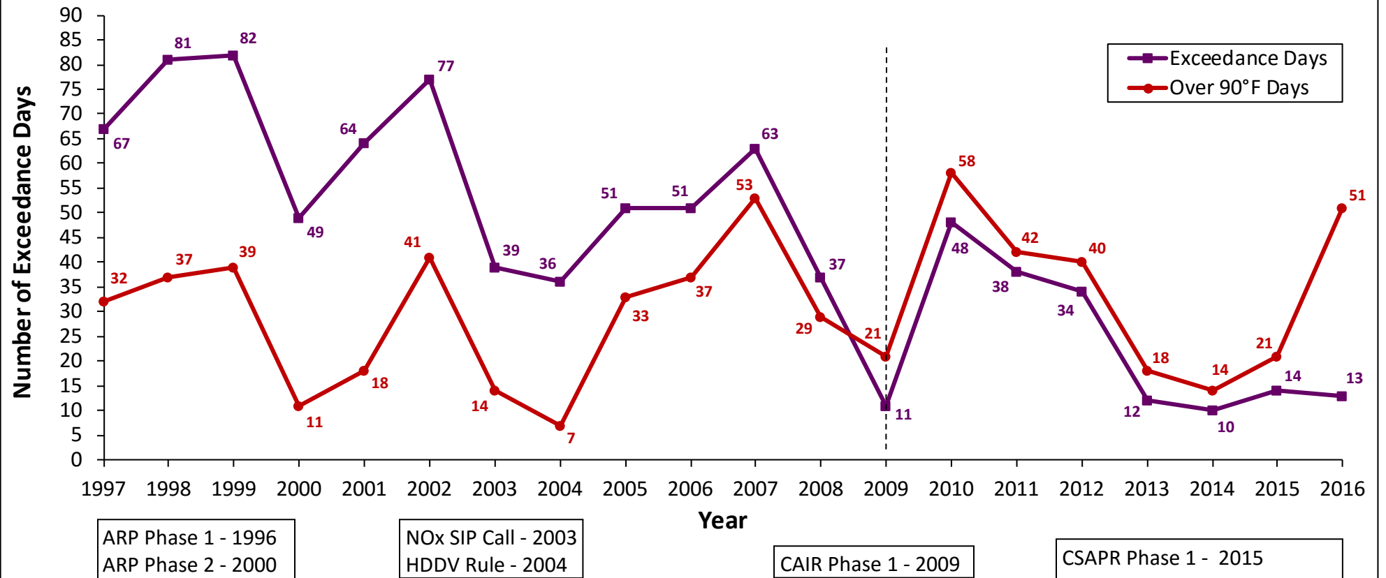
Figure 2: Over 90°F Days (Dulles) and 8-hour Ozone Exceedance Days (2015 std)
