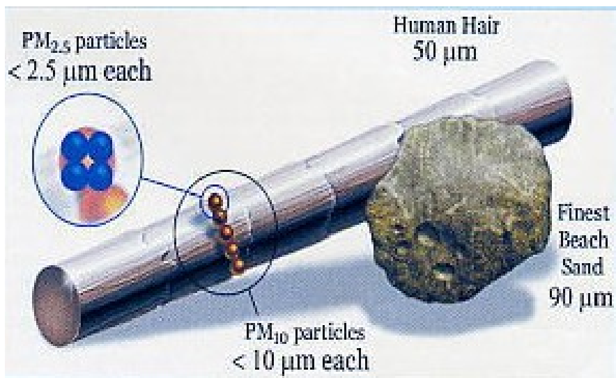
Figure 5: The Size of Particulate Matter
