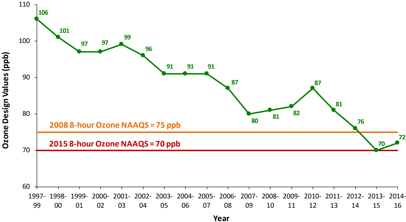
Figure 4: 8-hour Ozone Design Values in the DC-MD-VA Nonattainment Area (1999-2016)
