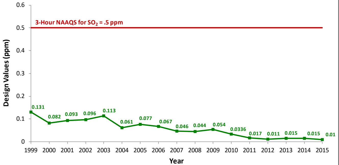
Figure 13: 3-Hour Design Values for Sulfur Dioxide (Washington, D.C. Region, 1999 - 2015)
