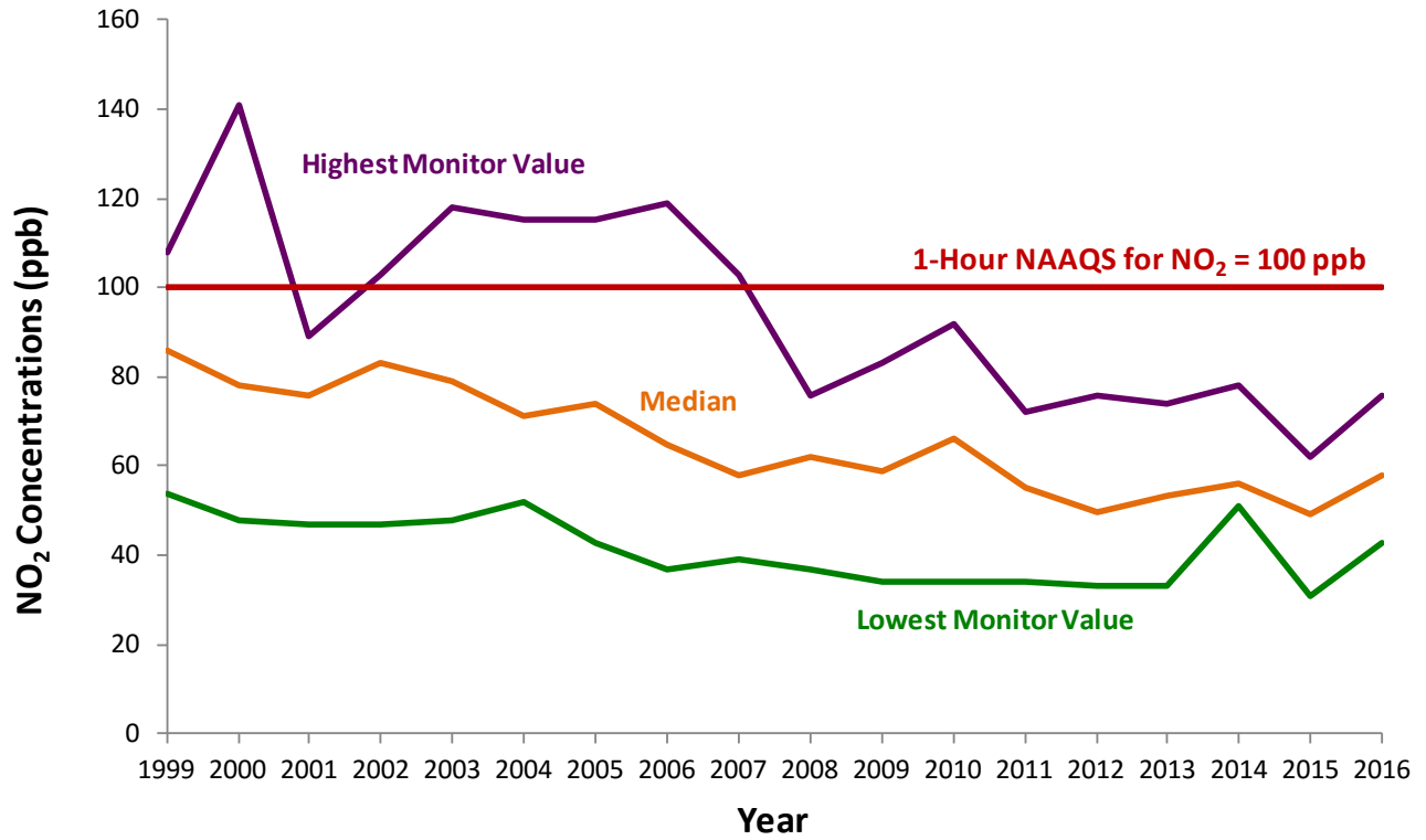
Figure 16: Maximum 1-Hour Monitor Concentrations for Nitrogen Dioxide (Washington, D.C. Region, 1999-2016)
