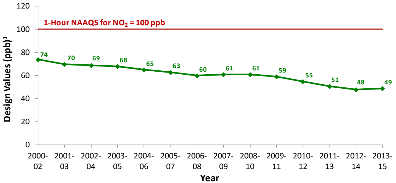
Figure 14: 1-Hour Design Values for Nitrogen Dioxide (Washington, D.C. Region, 2002-2015)
