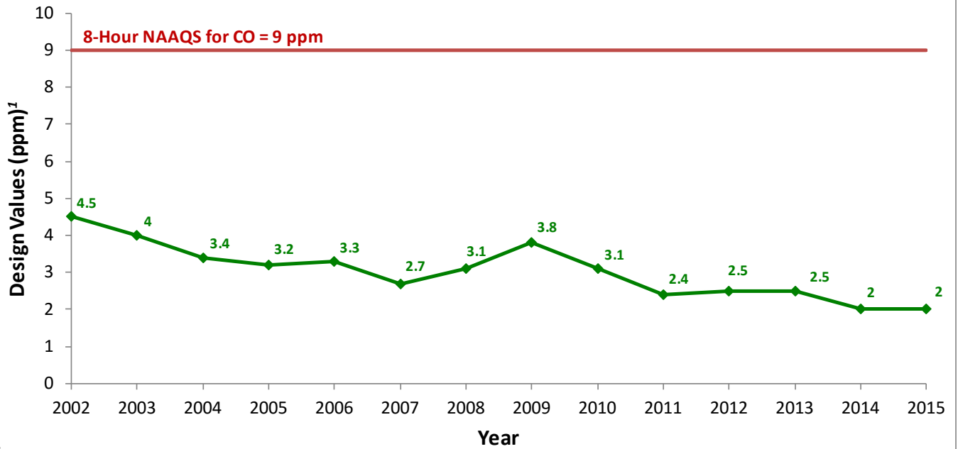
Figure 11: 8-Hour Design Values for Carbon Monoxide (Washington, D.C. Region, 2002-2015)
