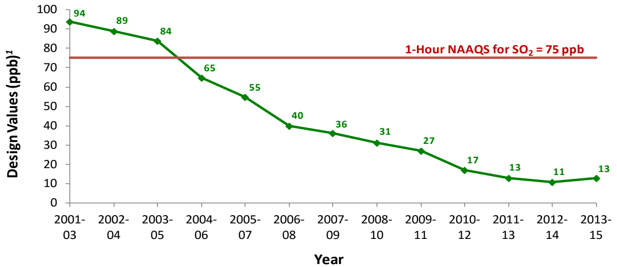
Figure 12: 1-Hour Design Values for Sulfur Dioxide (Washington, D.C. Region, 2003 - 2015)
