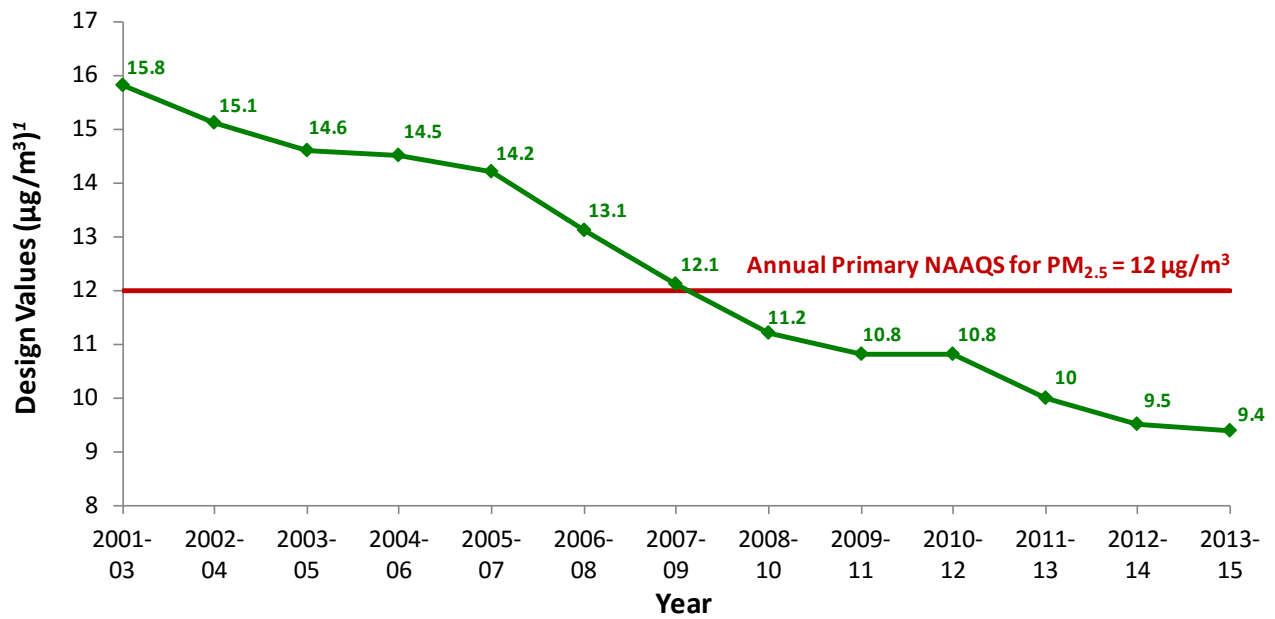
Figure 8: Annual Design Values for PM 2.5 (Washington, D.C. Region, 2003-2015)
