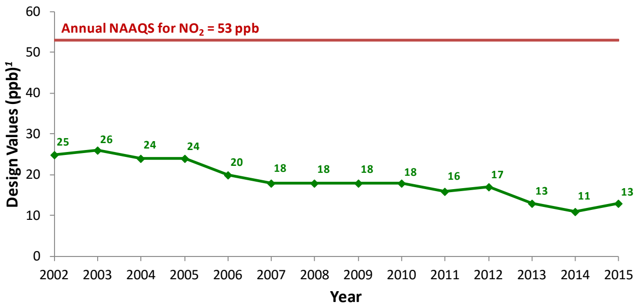
Figure 15: Annual Design Values for Nitrogen Dioxide (Washington, D.C. Region, 2002-2015)
