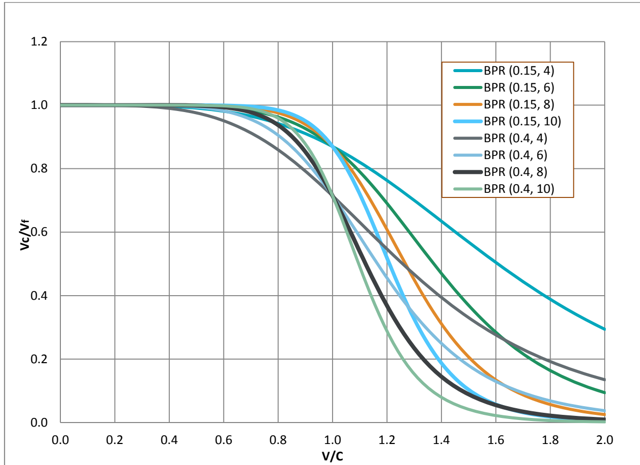
Figure 7 BPR Curves with Various Parameter Values
