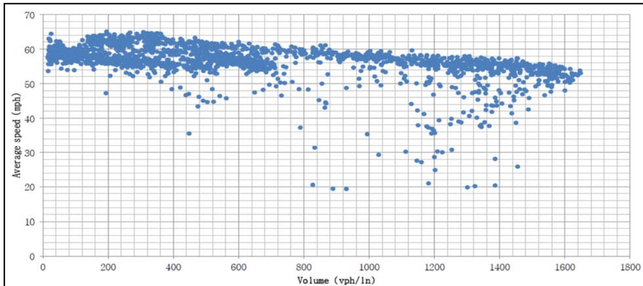
Figure 2 Scattergram of Observed Speed-Volume Data on a Typical Freeway Facility
