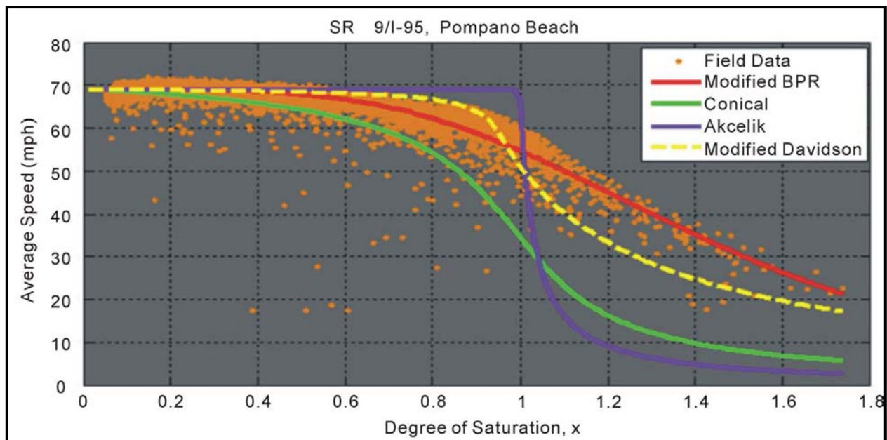
Figure 4 Fitted Volume-Delay Functions with Observed Data on a Freeway Segment
