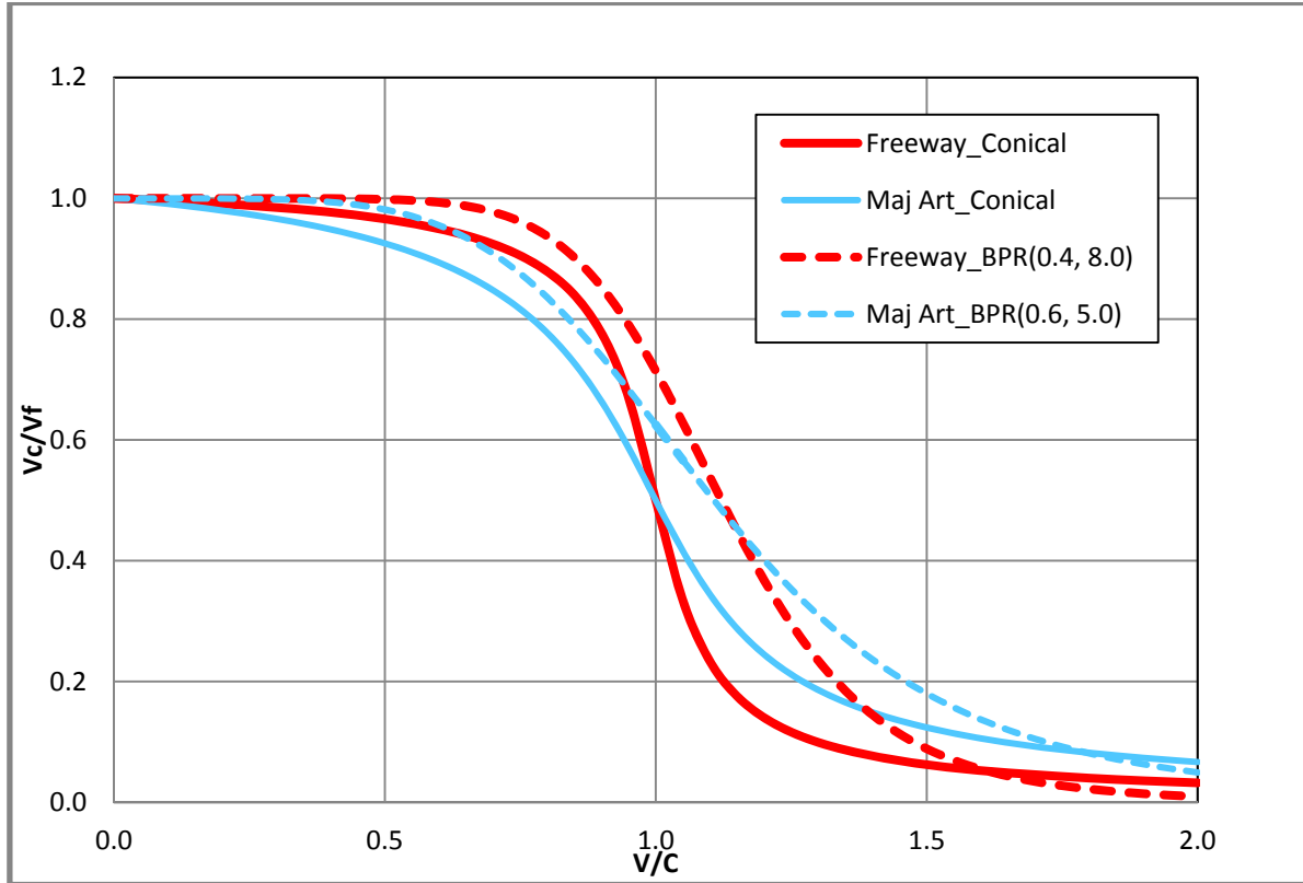
Figure 8 Comparison the Existing Conical Functions and Suggested BPR Functions
