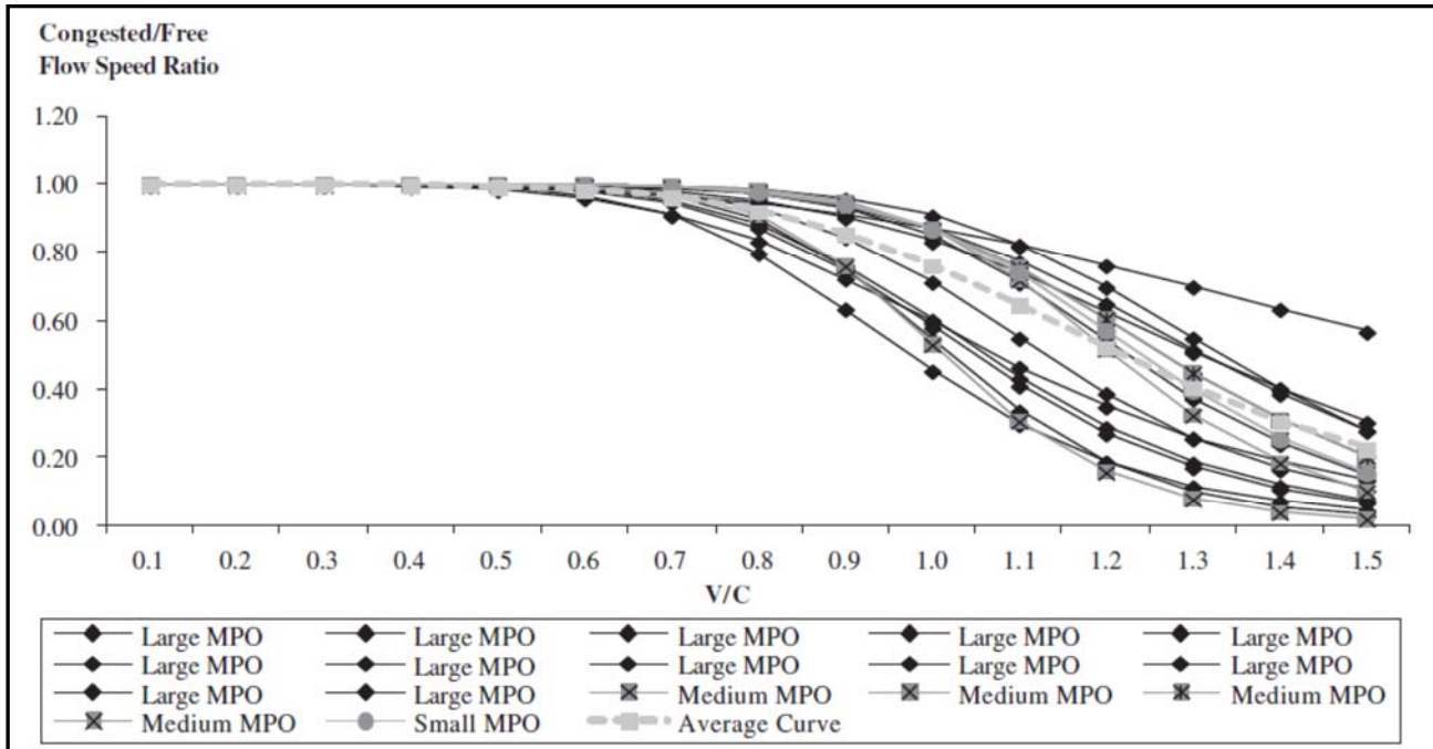
Figure 5 Volume-Speed Curves of Various BRP functions of Existing MPO Models –
