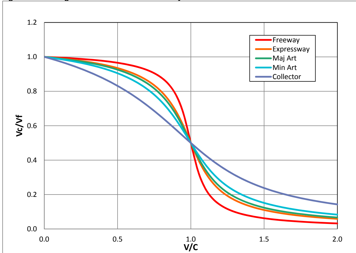
Figure 6 Existing MWCOG Model Volume-Delay Functions
