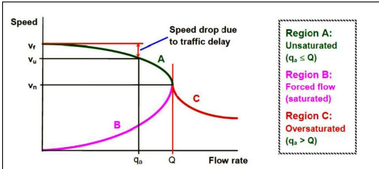
Figure 1 Speed-Flow Relationship Traffic Flow on Uninterrupted Flow Facilities
