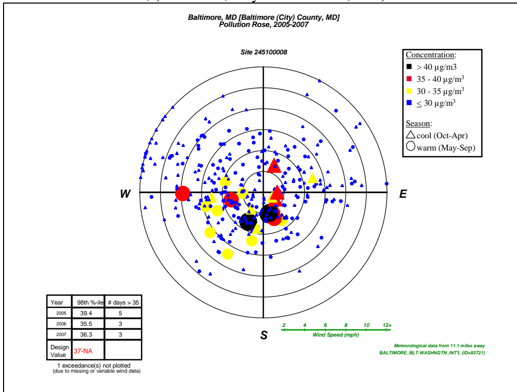
Figure 6.3. Pollution Rose for the City of Baltimore Monitor # 245100008, (SE Police, City of Baltimore, MD)
