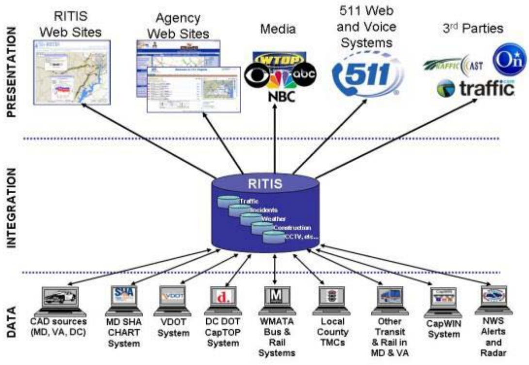
Figure 4: RITIS is a data integration and dissemination platform.
