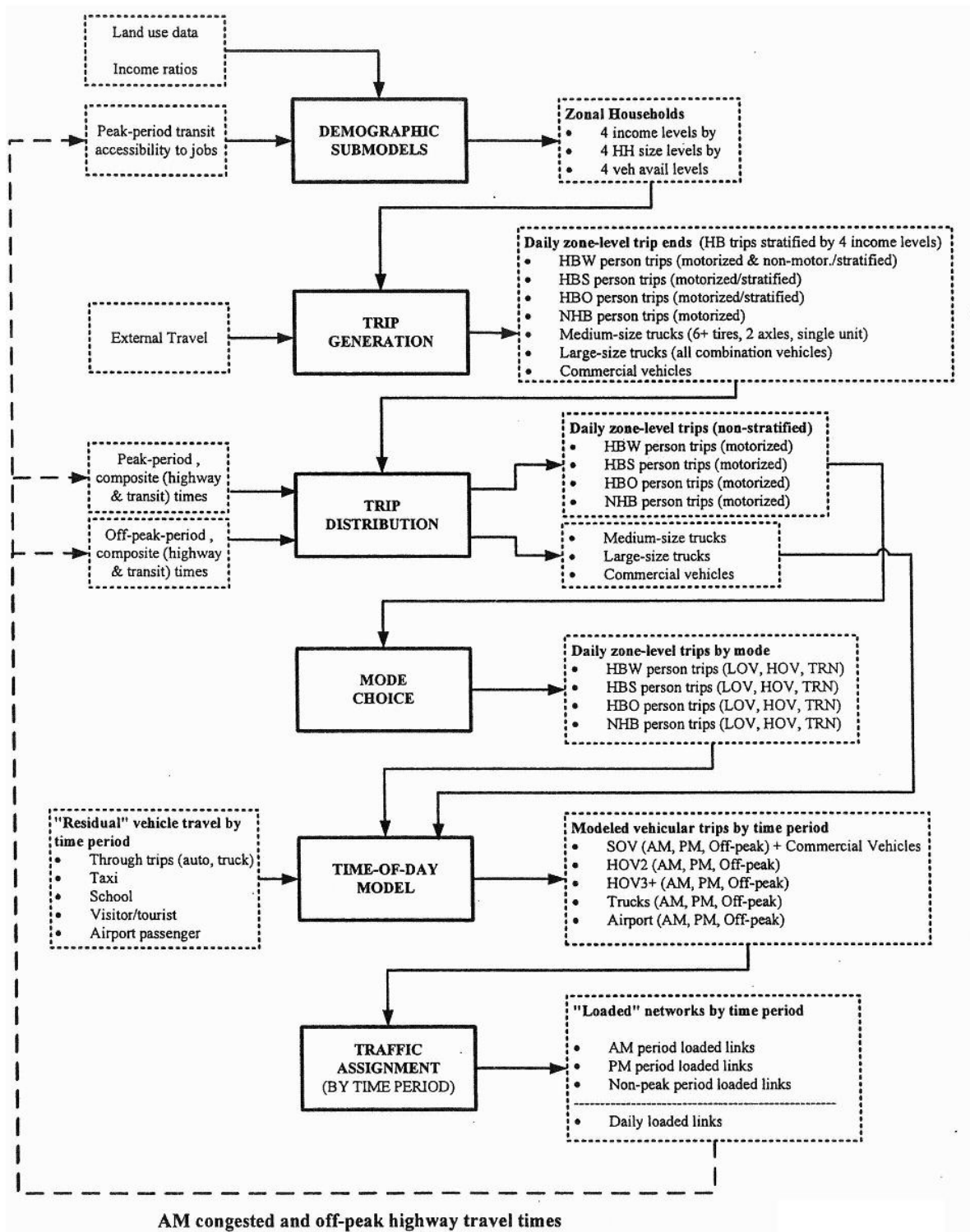
Figure 1. MWCOG/TPB Version 2.2 Model Structure
