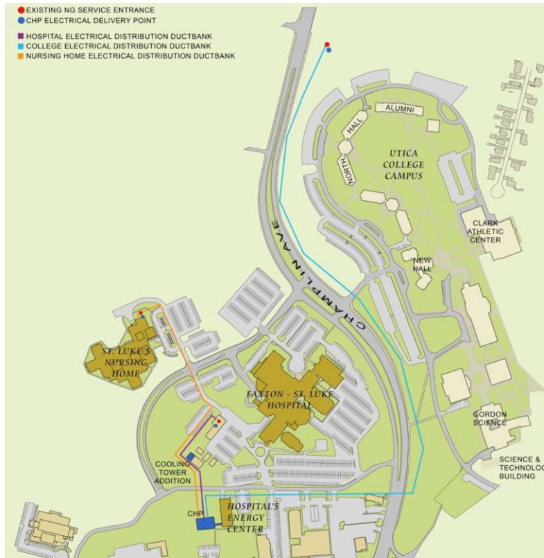
Map of New York's Burrstone Energy Center
