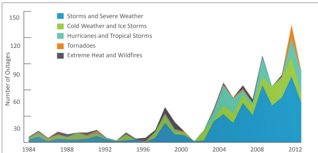
Outages of More than 50,000 Customers Caused by Extreme Weather
