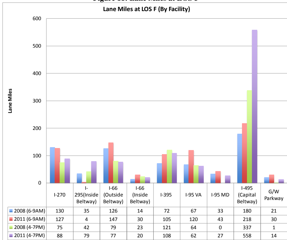
Figure 11: Lane Miles at LOS F
