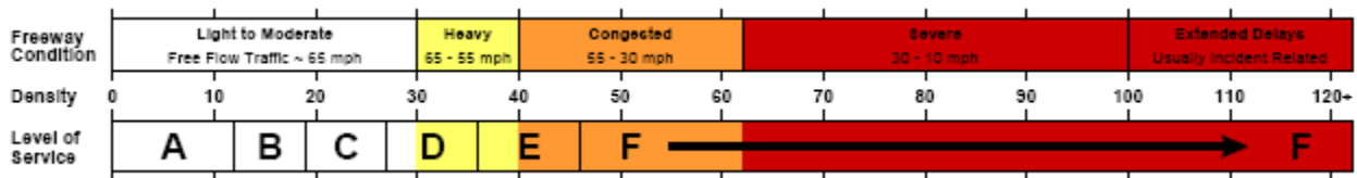
Figure 10: Speed, Density and LOS Chart
