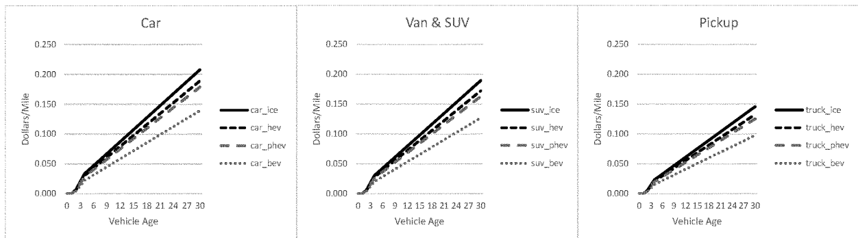
Figure 39. Repair cost per mile (2019 dollars) for a $35,000 car, van/SUV, and pickup with various powertrains
