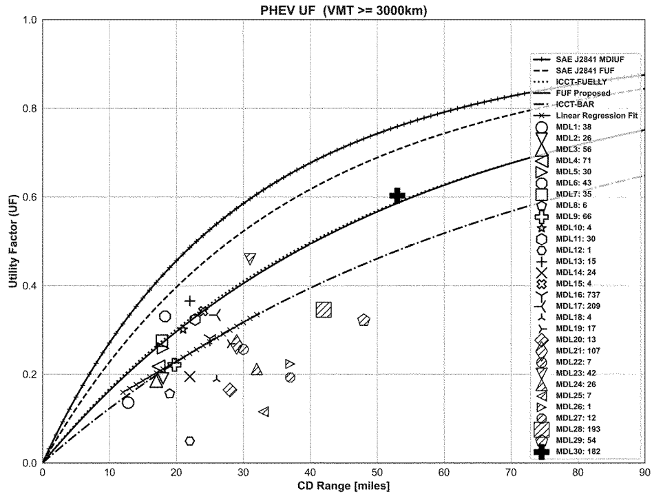
Figure 13. FUF proposed, SAE J2841 FUF and ICCT-BAR/FUELLY curves.
