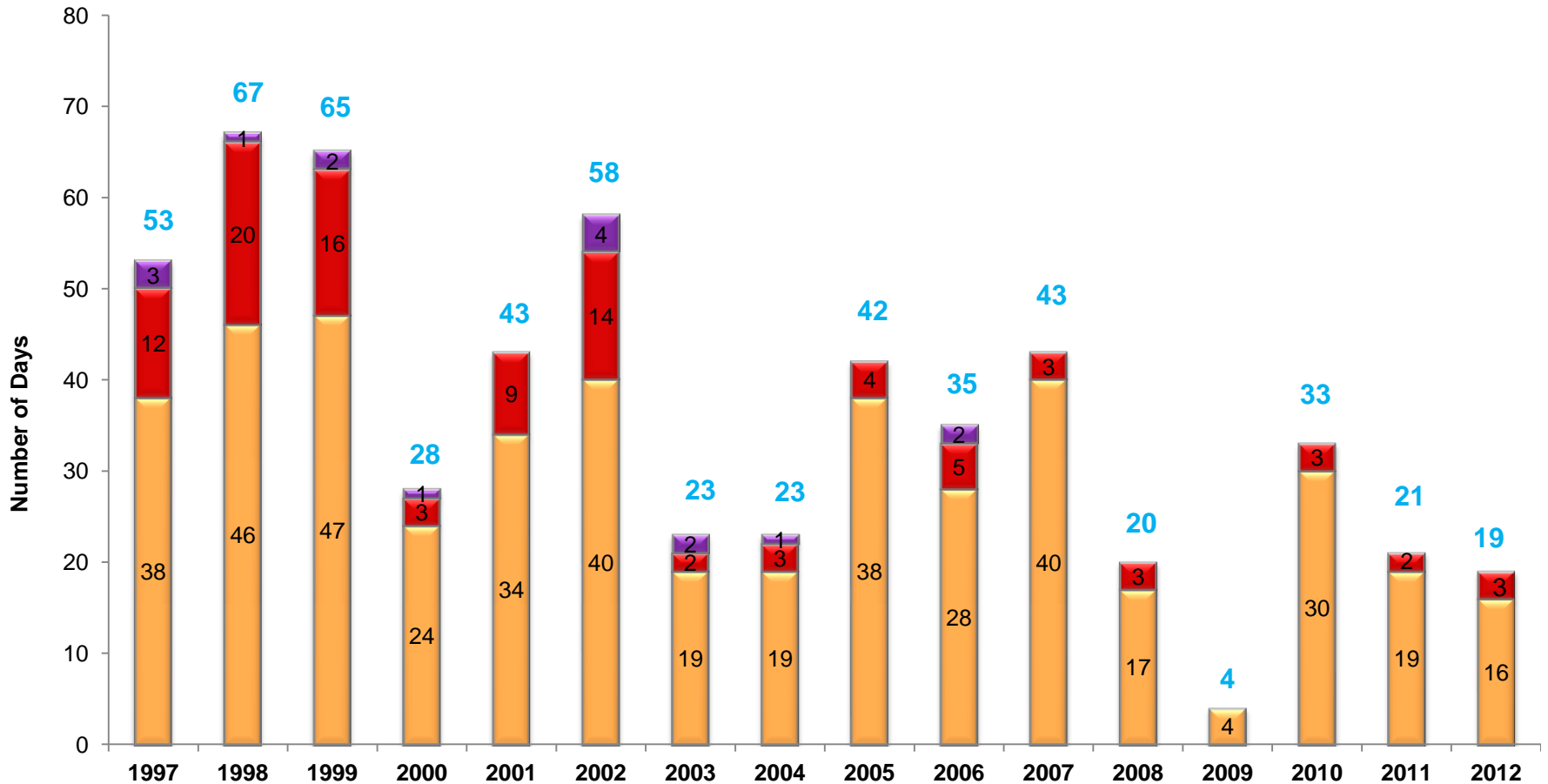
Number of Exceedance Days - 2008 Ozone Standard (75 ppb) Breakdown of Code Orange, Red, and Purple Days 1997 - 2012
