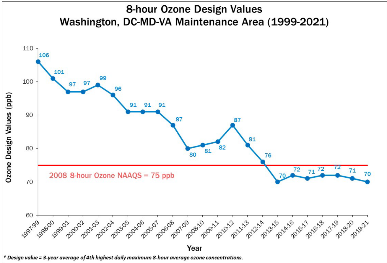
Figure 3-3: Ozone Design Value Trend
