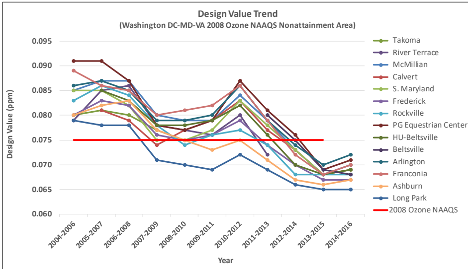
Figure 3-2: Washington DC-MD-VA Area Annual Ozone Data Trend
