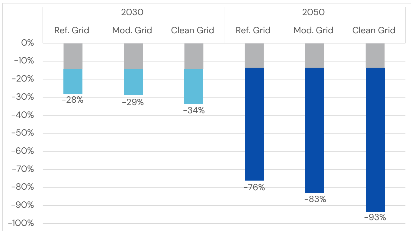
Figure 13. GHG Emission Reductions under VT.2 for the three different grid scenarios (Reference Case, Modified Reference Case, and Clean Grid Case)
