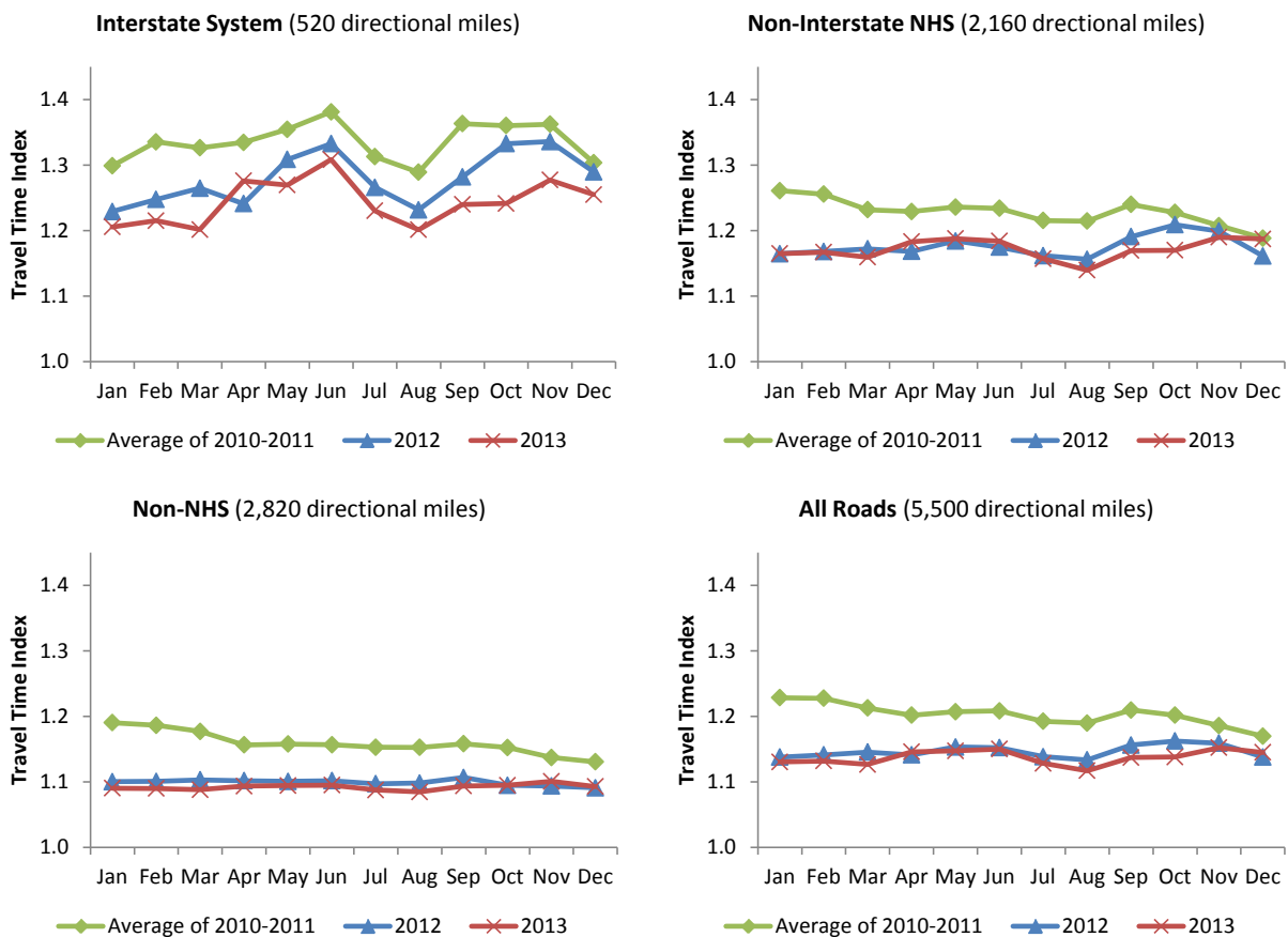
Figure 1. Monthly average Travel Time Index for AM peak (6:00-10:00 am) and PM peak (3:00-7:00 pm)
