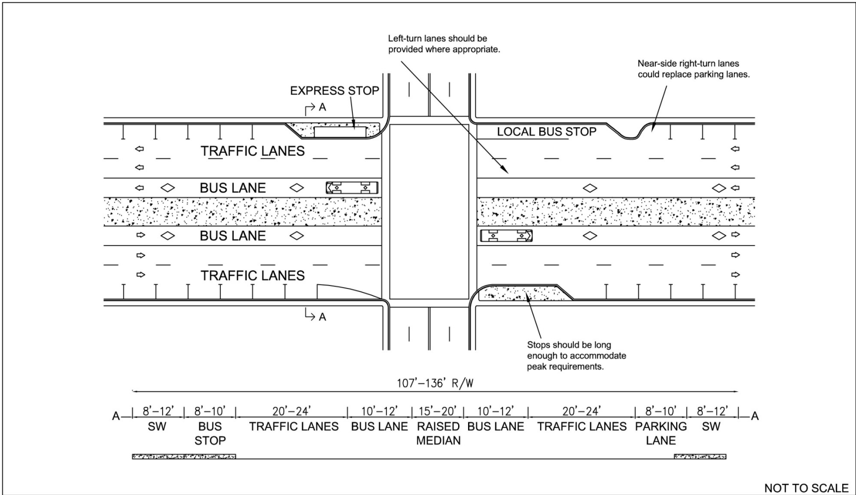
FIGURE 8: CENTER BUS LANE
