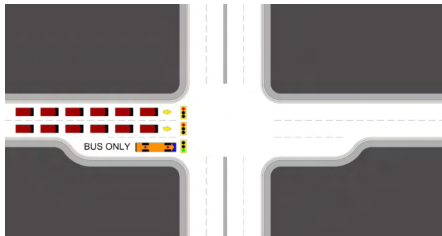
FIGURE 18: EXAMPLE OF QUEUE JUMPER WITH FAR-SIDE BUS BAY WITH TSP
