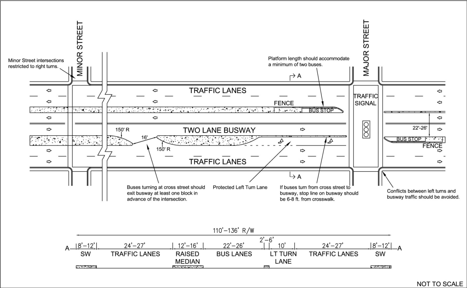
FIGURE 10: BUS LANE IN MEDIAN
