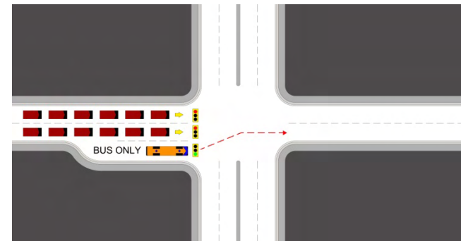
FIGURE 17: EXAMPLE OF QUEUE JUMPER WITH TSP
