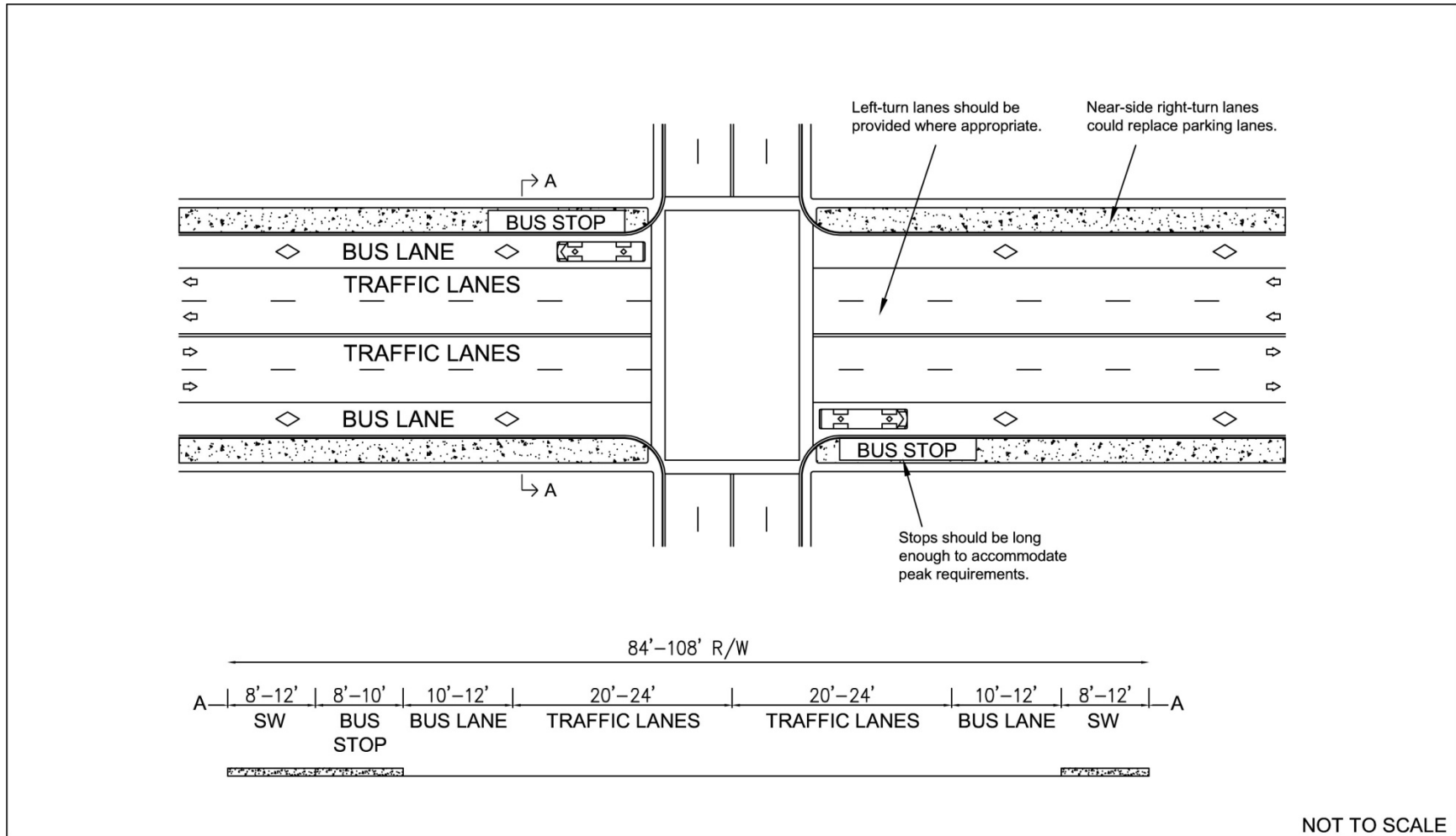
FIGURE 5: BUS LANE IN OUTSIDE LANE
