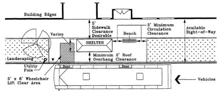
FIGURE 22: EXAMPLE OF BUS STOP & SHELTER DESIGN
