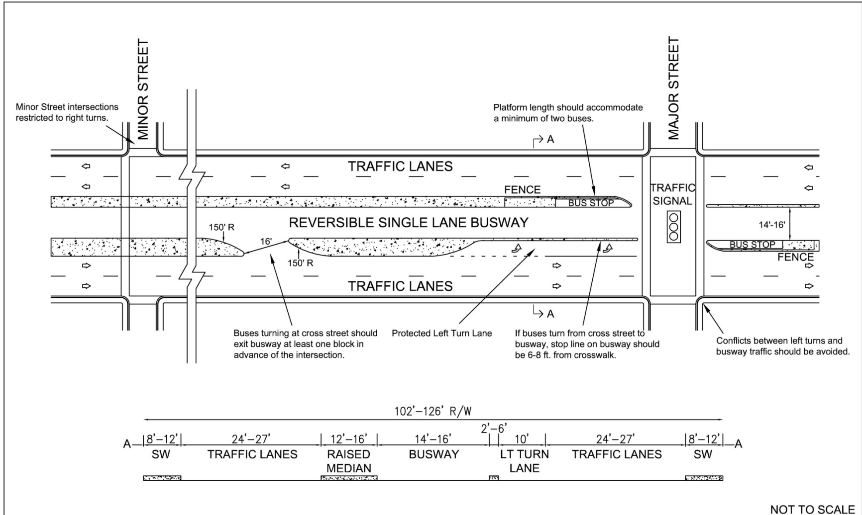
FIGURE 12: REVERSIBLE BUS LANE IN MEDIAN
