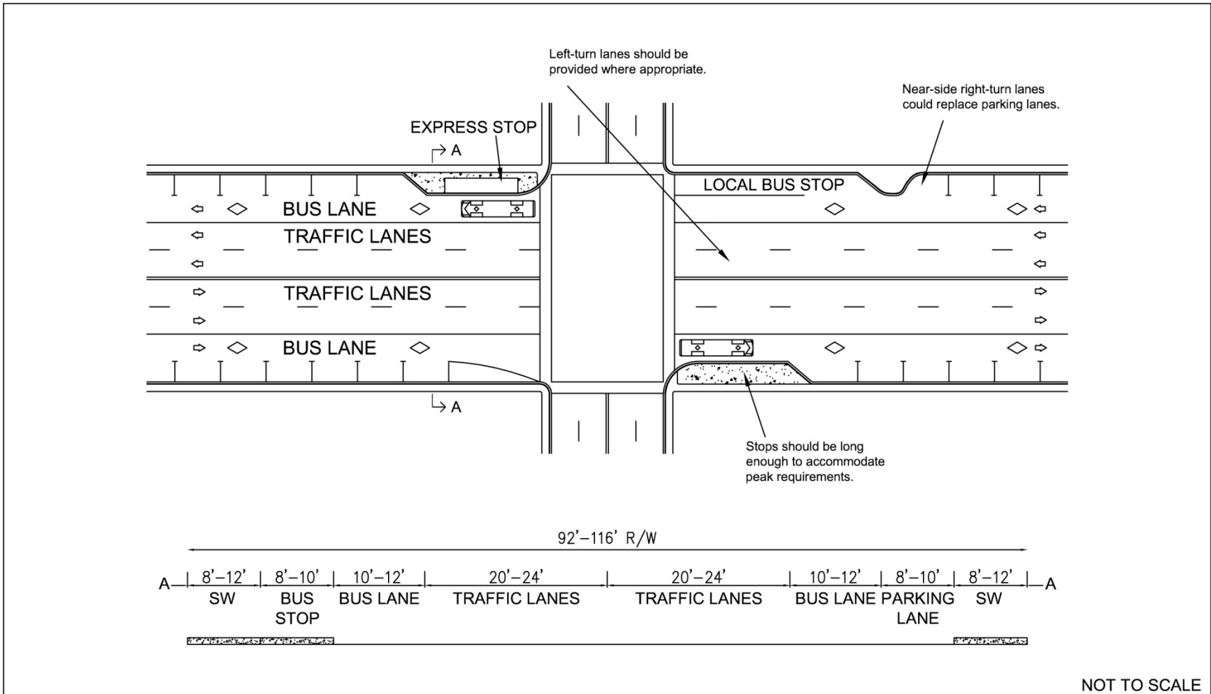
FIGURE 7: MIDDLE BUS LANE WITH ON-STREET PARKING
