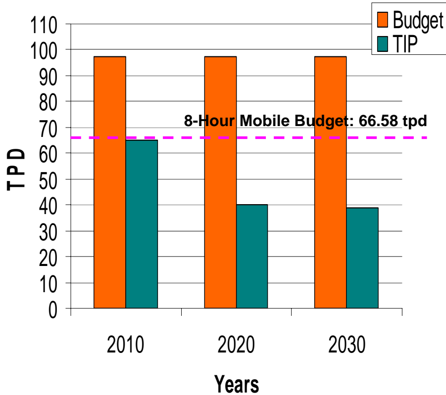
VOC Emissions for 2005 CLRP and 2006 TIP
