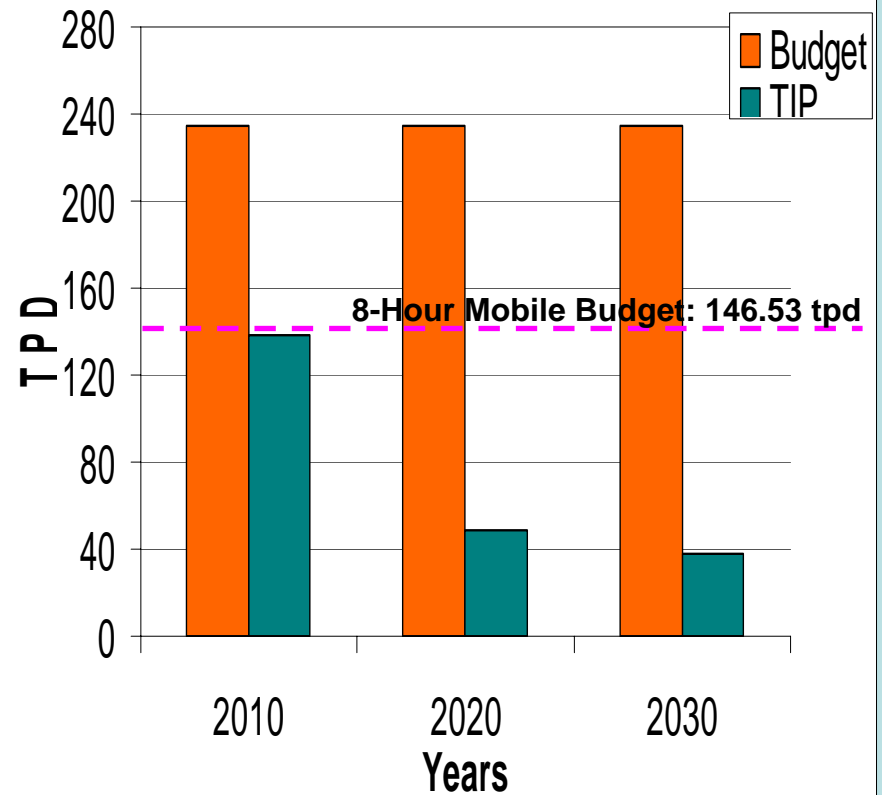
NOx Emissions for 2005 CLRP and 2006 TIP
