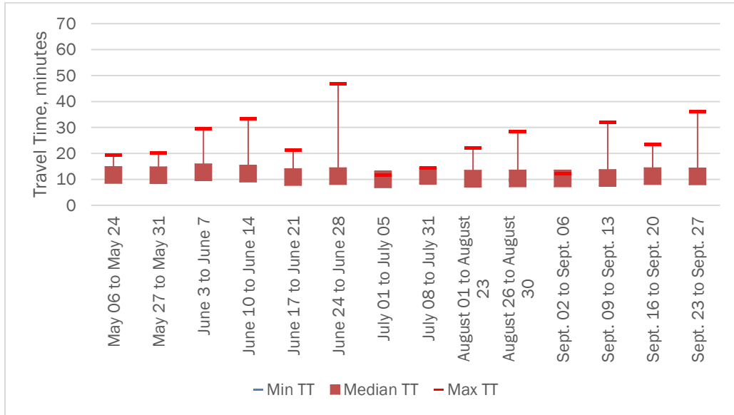
FIGURE 7 - MINIMUM, MEDIAN, AND MAXIMUM TRAVEL TIMES FOR THE GENERAL ROUTE USED BY SHUTTLE BUSES BETWEEN KING STREET AND NATIONAL AIRPORT STATIONS
