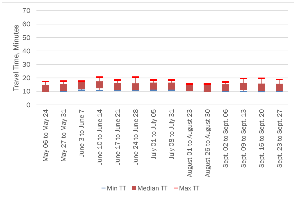
FIGURE 7 - MINIMUM, MEDIAN, AND MAXIMUM TRAVEL TIMES FOR THE GENERAL ROUTE USED BY SHUTTLE BUSES BETWEEN KING STREET AND NATIONAL AIRPORT STATIONS
