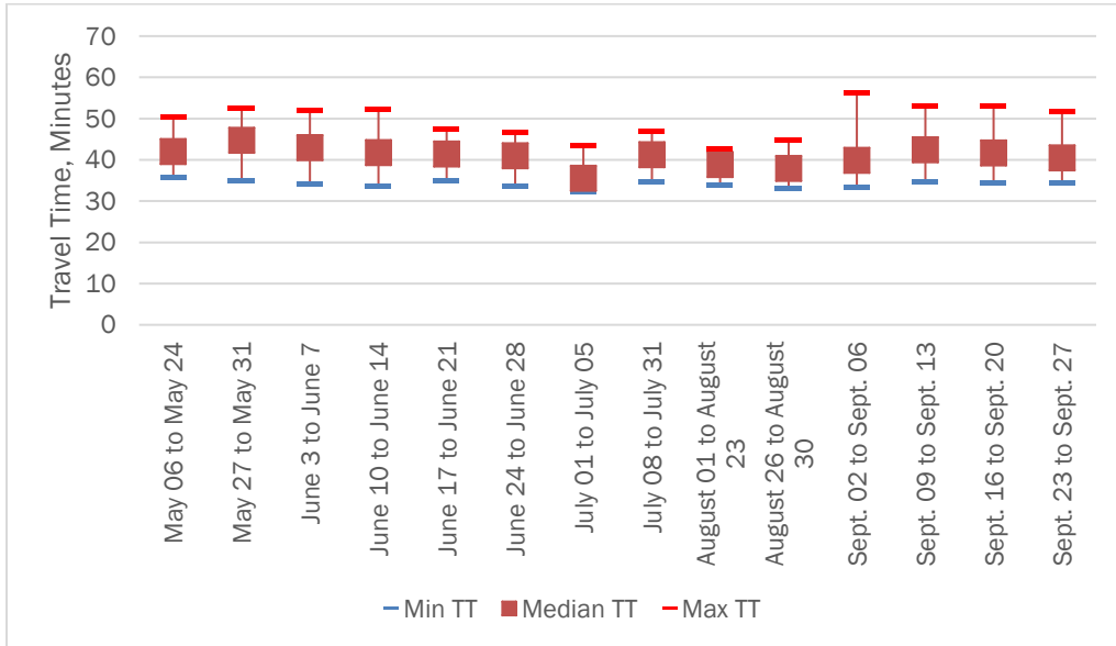
FIGURE 3 - MEDIAN, MINIMUM, AND MAXIMUM TRAVEL TIMES FOR THE US 1 CORRIDOR
