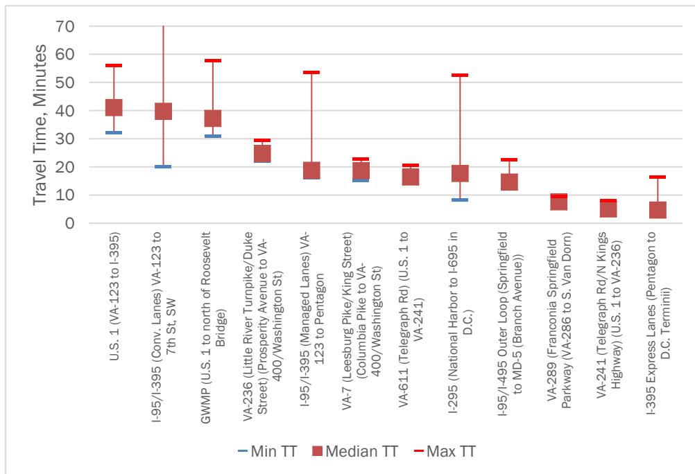
FIGURE 4 - MAJOR CORRIDORS TRAVEL TIMES DURING FULL SHUTDOWN PERIOD 5
