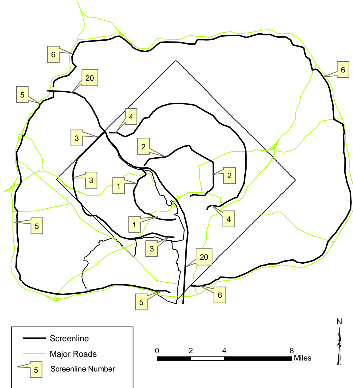
Figure 3-13 Highway Network screenlines: Inside the Beltway
