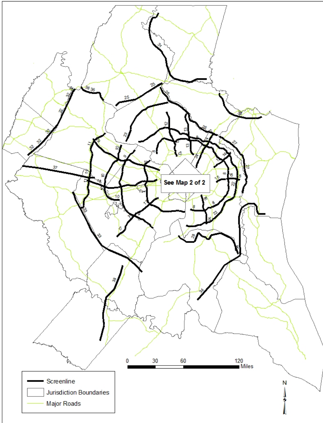
Figure 3-14 Highway network screenlines: Outside the Beltway
