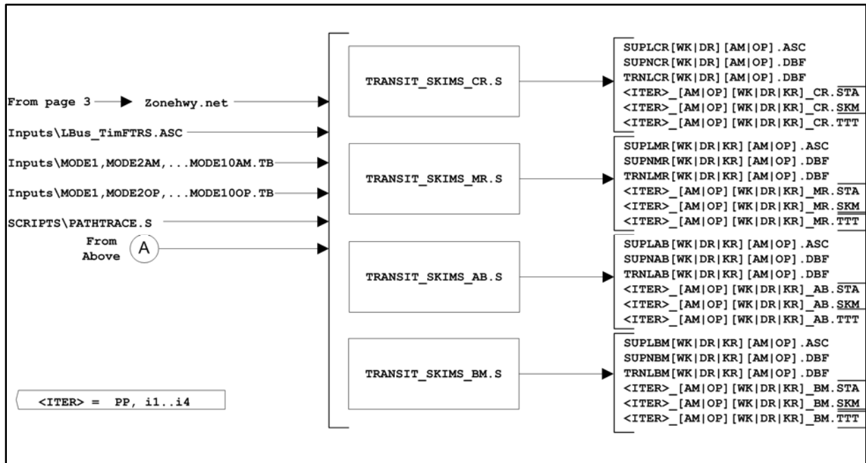
Figure 3-25 Process for conducting transit path building
