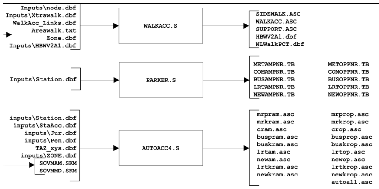
Figure 3-15 Process for developing walk-access and drive-access links
