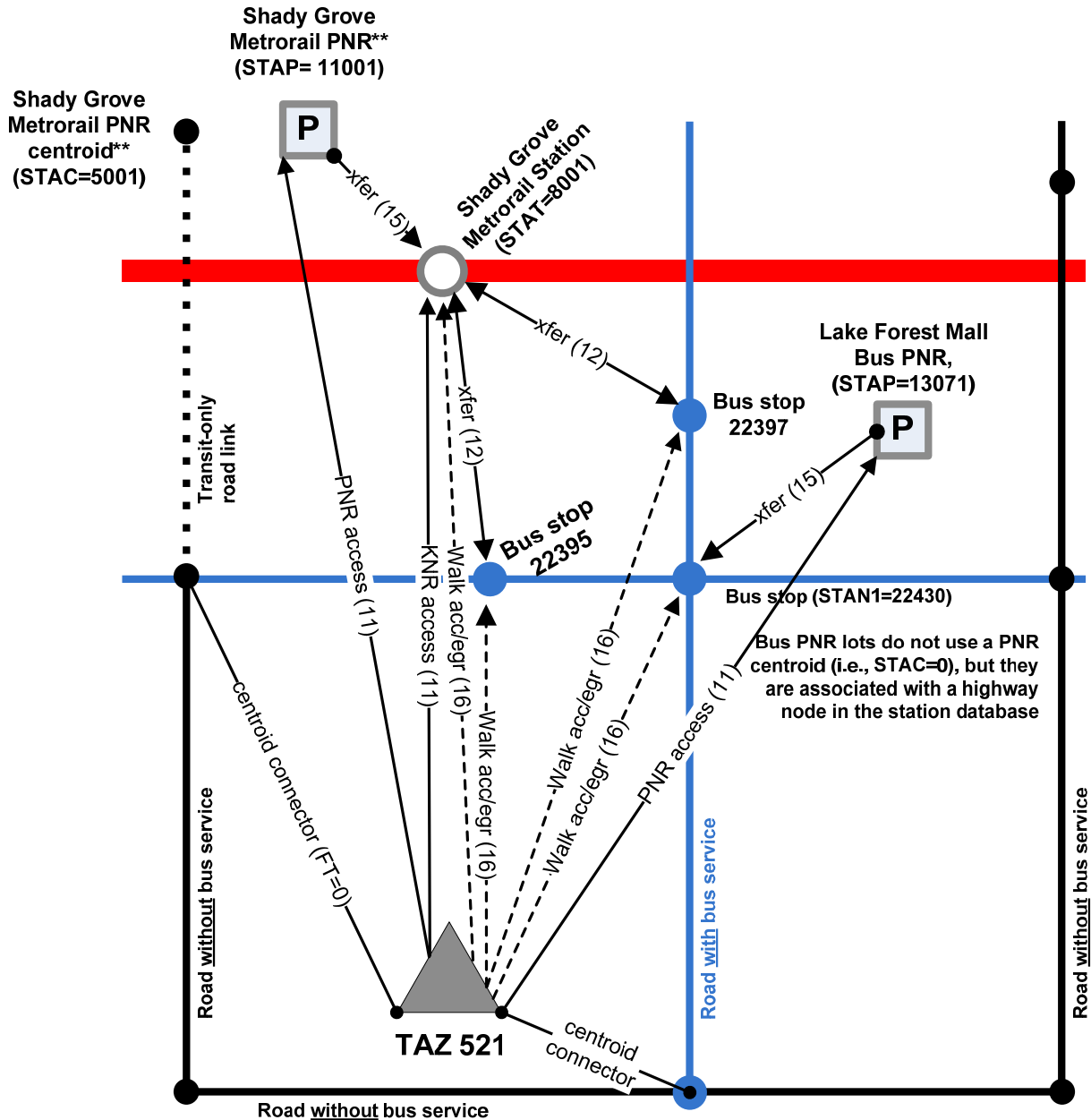
Figure 3-24 Existing MWCOC/TRNBUILD convention for network coding around rail stations, park-and-ride lots, and bus service
