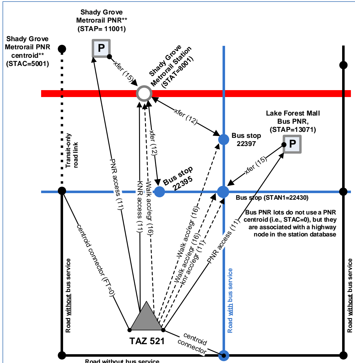
Figure 3-23 Existing MWCOC/TRNBUILD convention for network coding around rail stations, park-and-ride lots, and bus service
