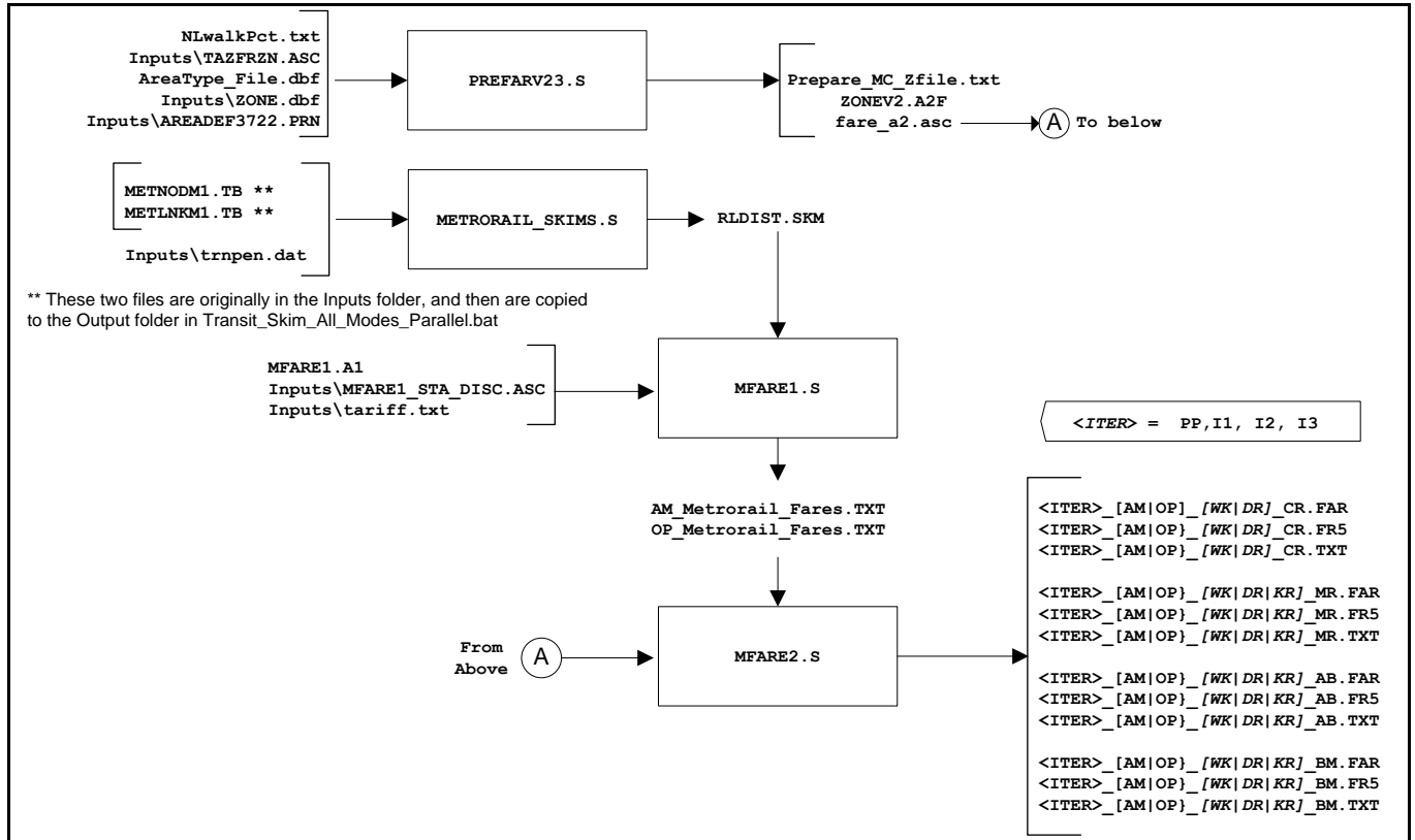
Figure 3-29 Process for developing zone-to-zone transit fares
