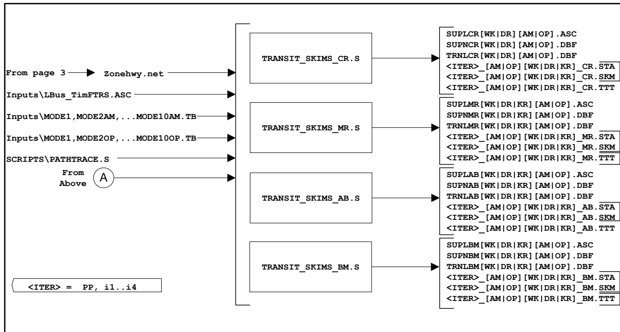
Figure 3-24 Process for conducting transit path building
